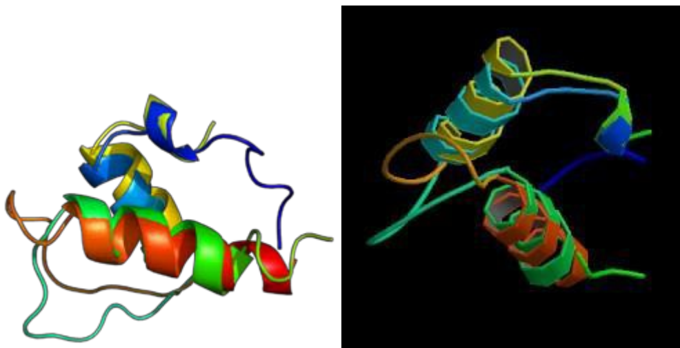
Figure 3. 3D structure of thymopoietin (source: Wikipedie)
